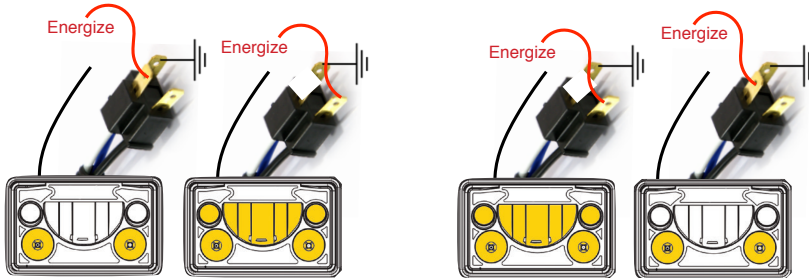
DOT High Beam
